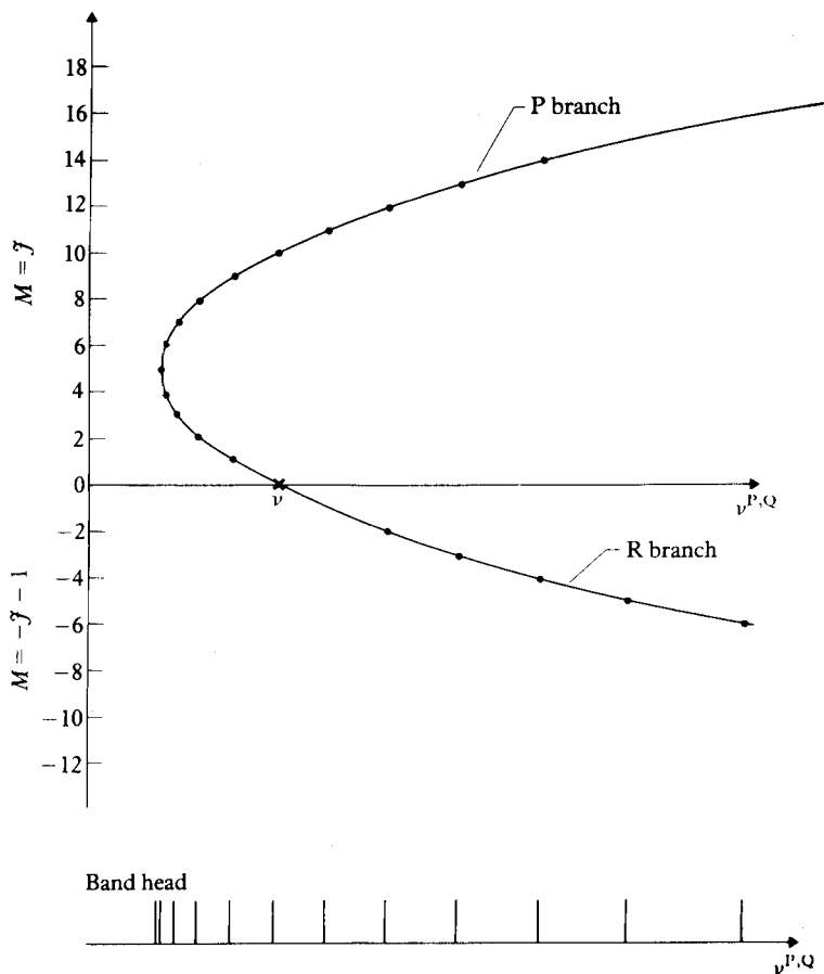
10.9 A Fortrat parabola for a \Sigma \rightarrow \Sigma transition in a diatomic molecule, (no Q branch). The spectrogram beneath shows the position of the band head.
